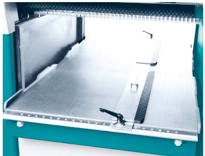
Second Second feather board for profiling work
