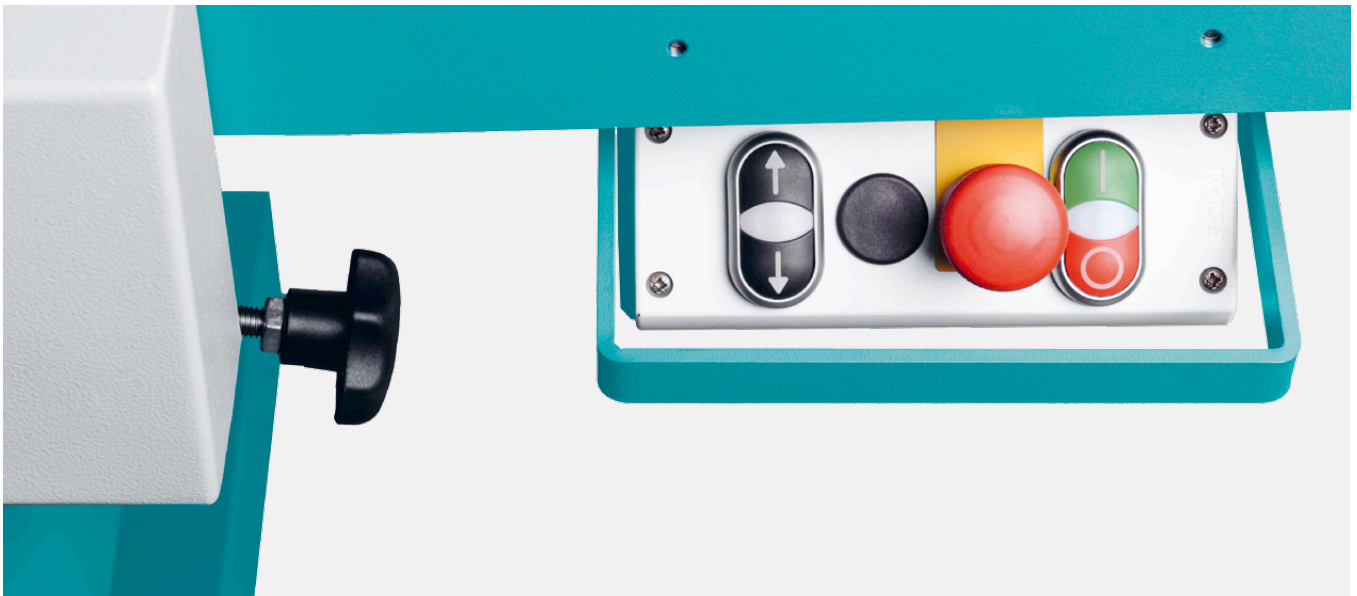
Control desk under infeed table
