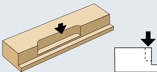
Spindle for vertical routing from the top (hinges grooving and glazing bead cut-off)
